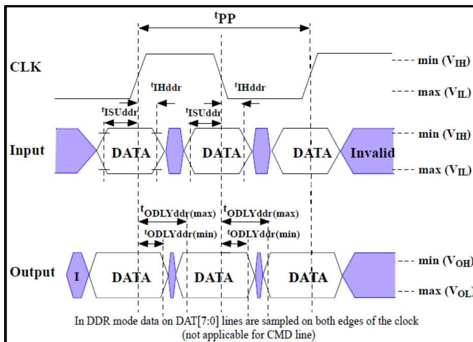
Figure 6.8 – Timing Diagram: Data Input/Output in Dual Data Rate Mode
