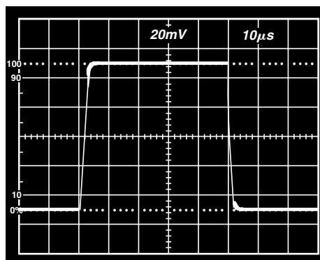
TPC 22. Small Signal Pulse Response, G = 100 , R_L = 2 k\Omega , C_L = 100 pF
