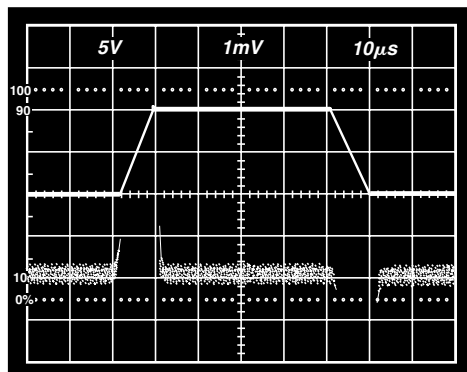
TPC 19. Large Signal Pulse Response and Settling Time Gain, G = 10 ( 0.5 mV = 0.01\% ), R_L = 1 k\Omega , C_L = 100 pF
