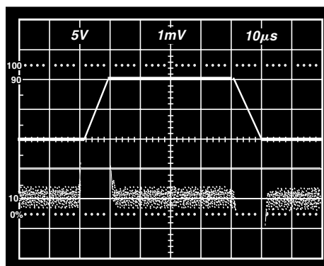
TPC 21. Large Signal Pulse Response and Settling Time, G = 100 ( 0.5 mV = 0.1\% ), R_L = 2 k\Omega , C_L = 100 pF
