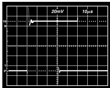
TPC 20. Small Signal Pulse Response, G = 10 , R_L = 1 k\Omega , C_L = 100 pF
